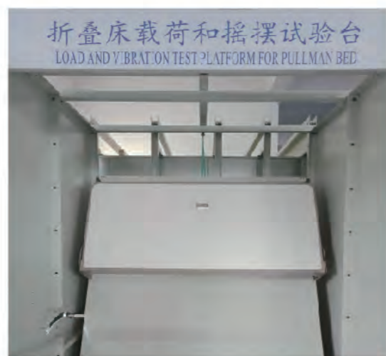
摇摆试验 | Vibration Test
