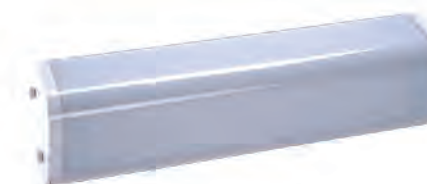
LED/荧光 走道灯 LED/Fluorescent corner light 型号/Type:JBL7-1(7W-LED) JBY15-1(15W-荧光/Fluorescent) 尺寸/Size:673x125x125(mm) 防护等级/Protection class:IP44
